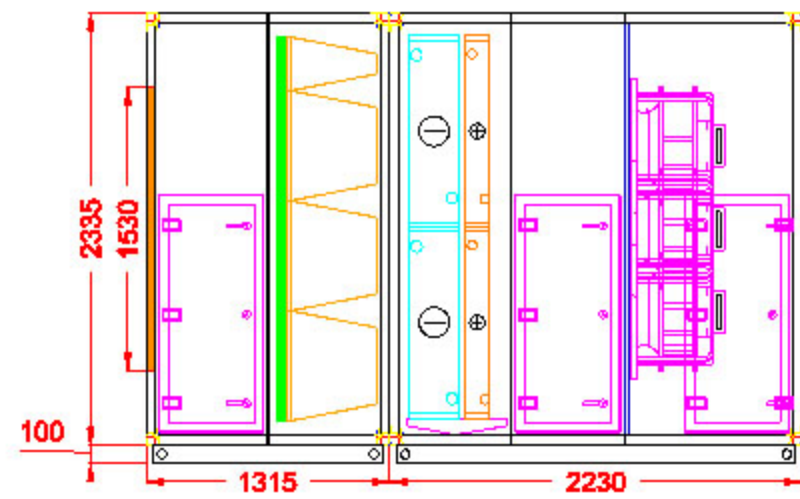
Right View
