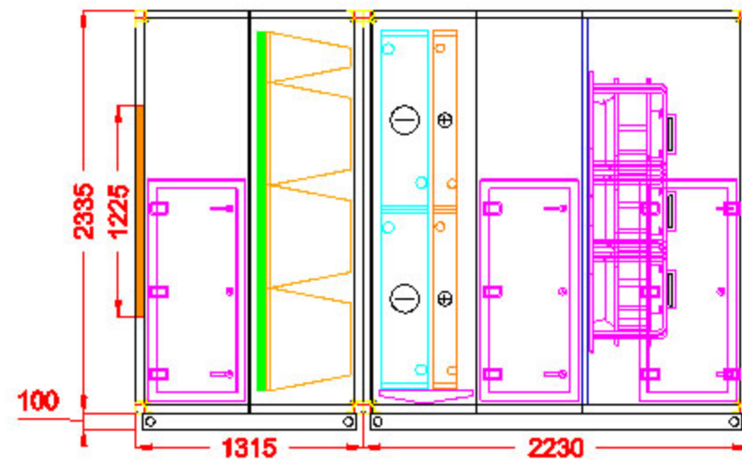
Right View
