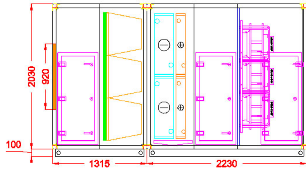
Right View
