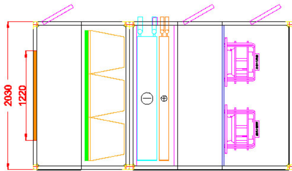
Top View
