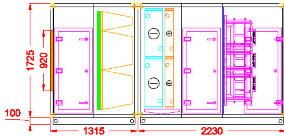
Right View
