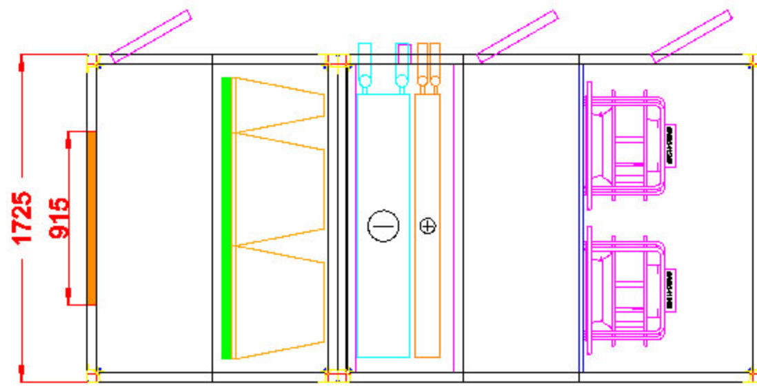
Top View
