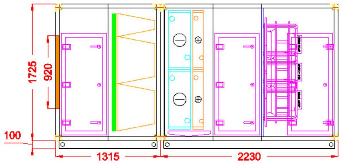
Right View
